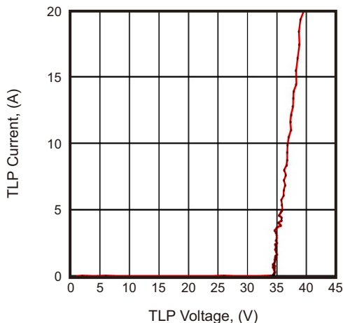
Fig.5 - TLP-Positive Pulse
